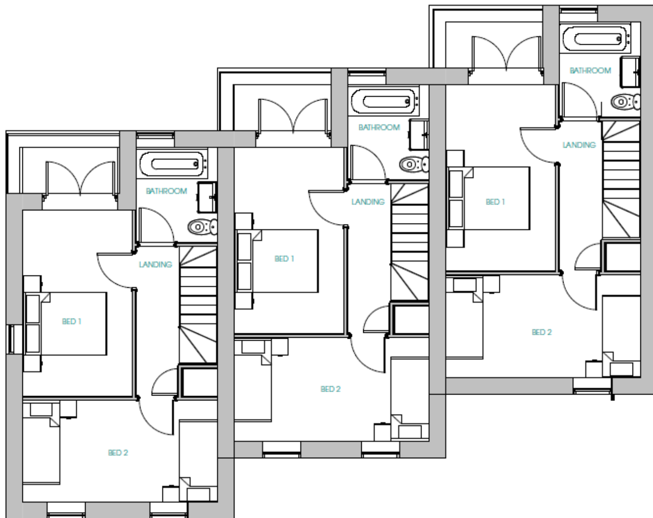
PLOTS 3-5 - 2 BEDROOM TERRACE FIRST FLOOR PLAN
